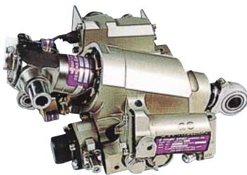
B777 AILERON POWER CONTROL UNIT
