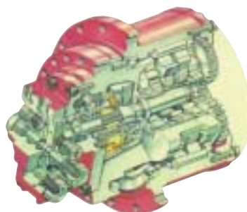
Cross-section of a reduction drive
